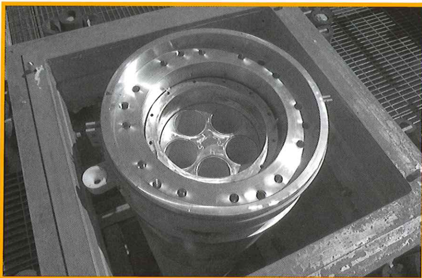
SNF container with the lid removed, showing view of internal basket
